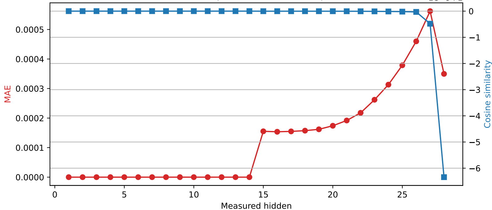
Qwen2.5-7B-Instruct | Quantized layer 14 | float32 → int16
