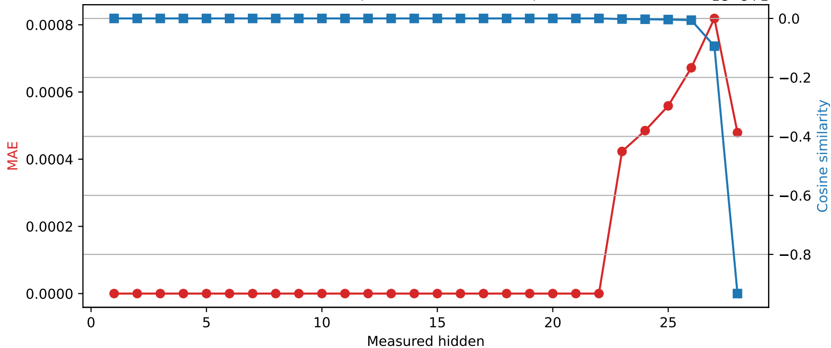
Qwen2.5-7B-Instruct | Quantized layer 22 | float32 → int16
