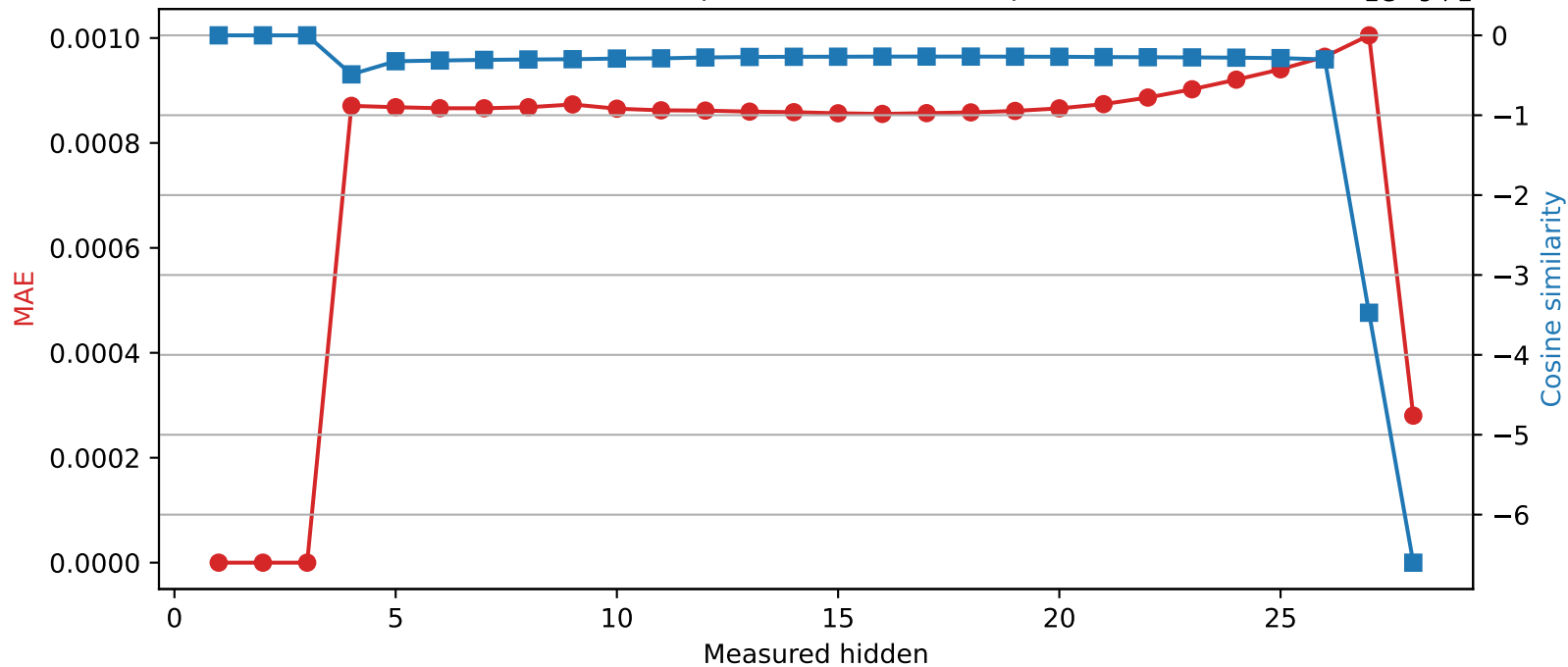
Qwen2.5-7B-Instruct | Quantized layer 3 | float32 → int16
