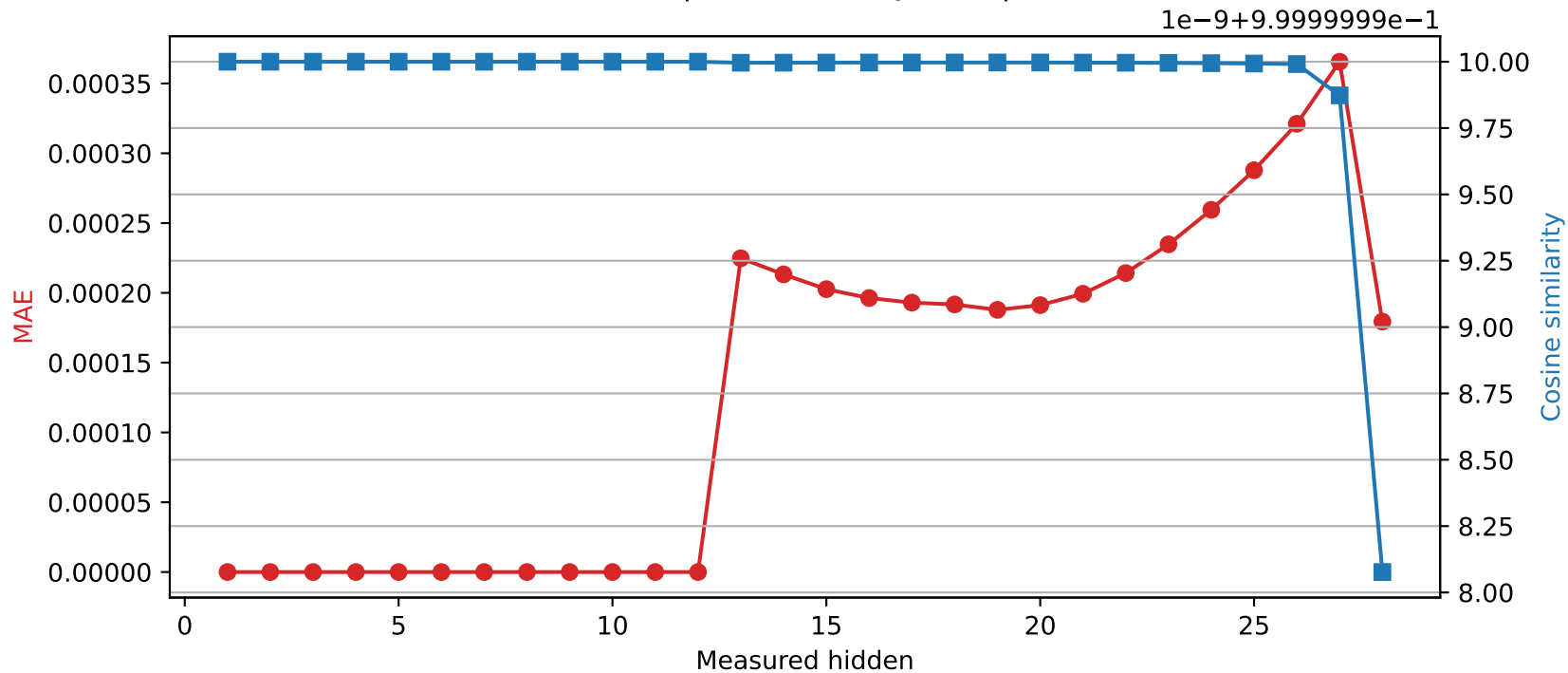
Qwen2.5-7B-Instruct | Quantized layer 12 | float32 \rightarrow int16
