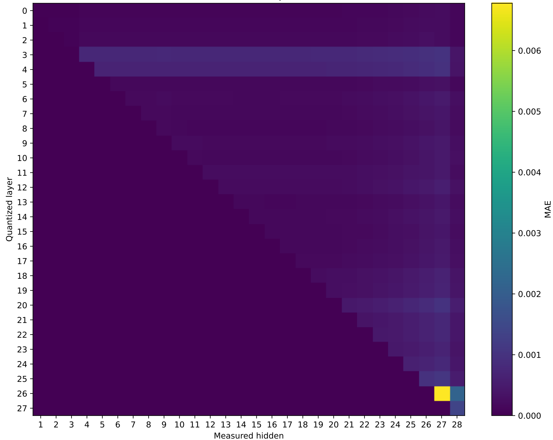
Model: Qwen2.5-7B-Instruct | float64 → int16
