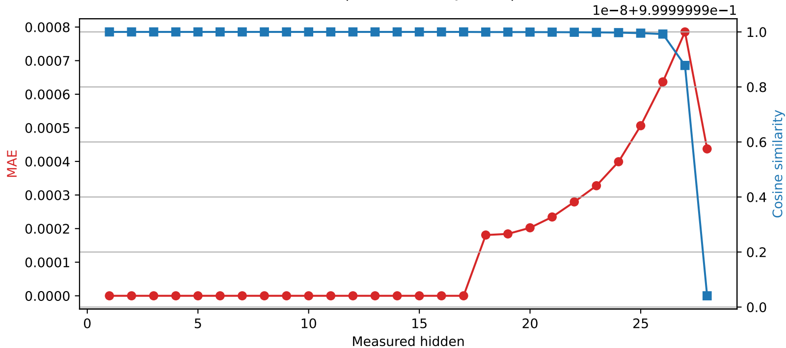
Qwen2.5-7B-Instruct | Quantized layer 17 | float64 → int16
