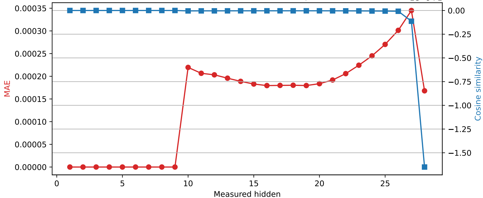
Qwen2.5-7B-Instruct | Quantized layer 9 | float64 → int16
