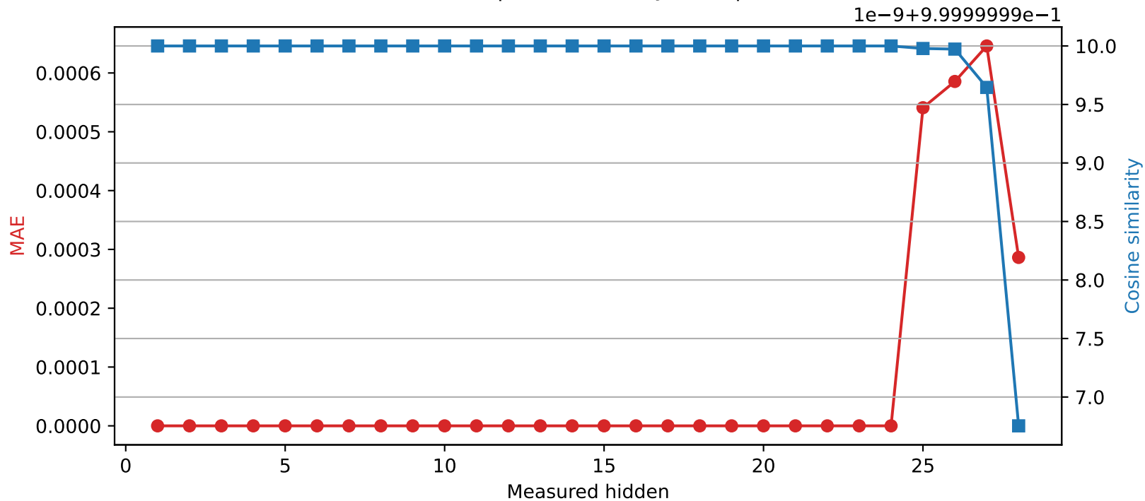
Qwen2.5-7B-Instruct | Quantized layer 24 | float64 → int16
