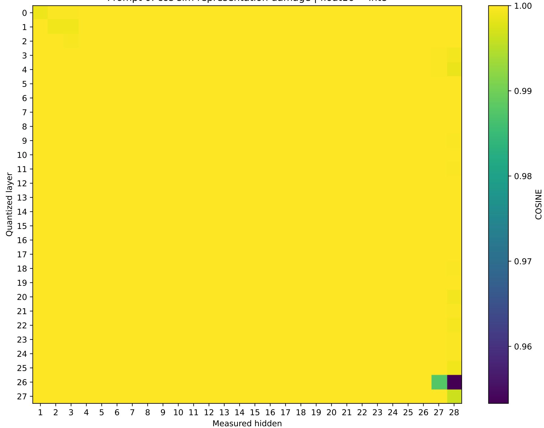
Qwen2.5-7B-Instruct Prompt 0: cos sim representation damage | float16 → int8
