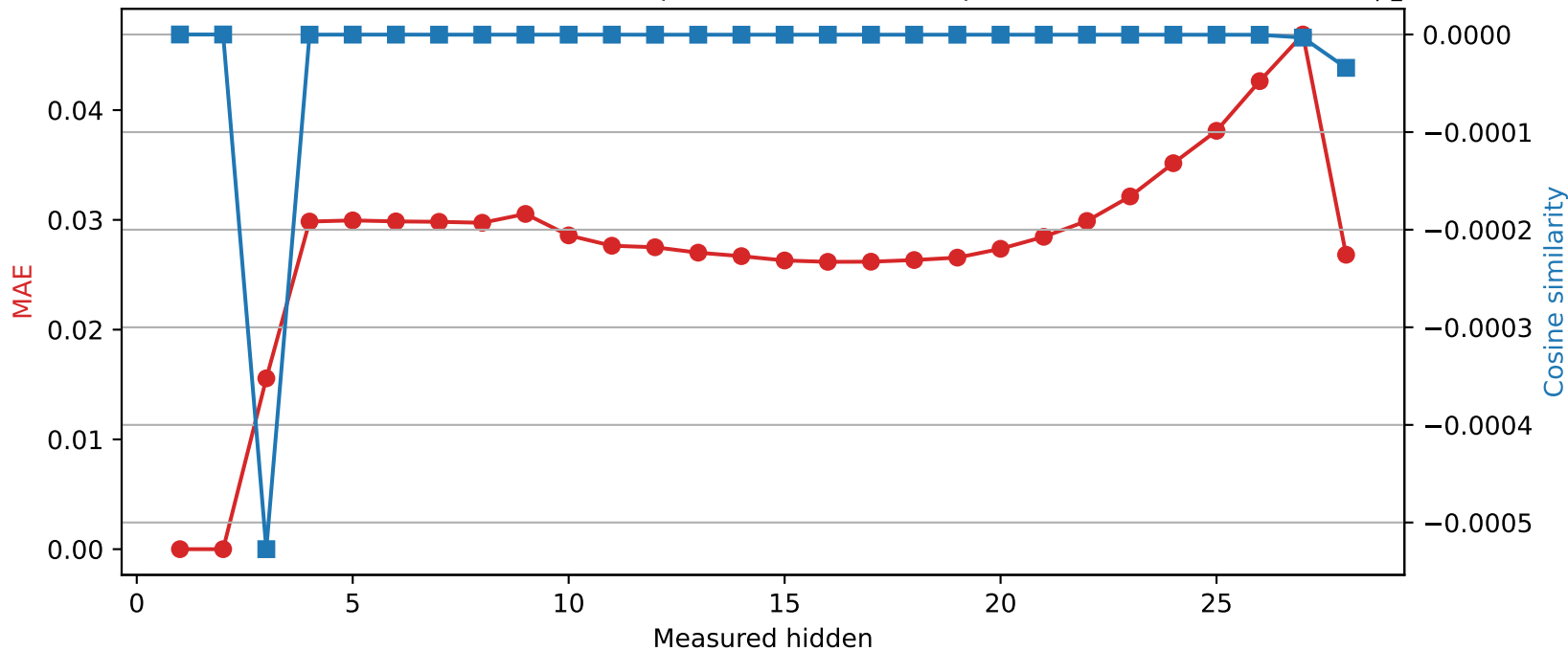
Qwen2.5-7B-Instruct | Quantized layer 2 | float16 \rightarrow int8
