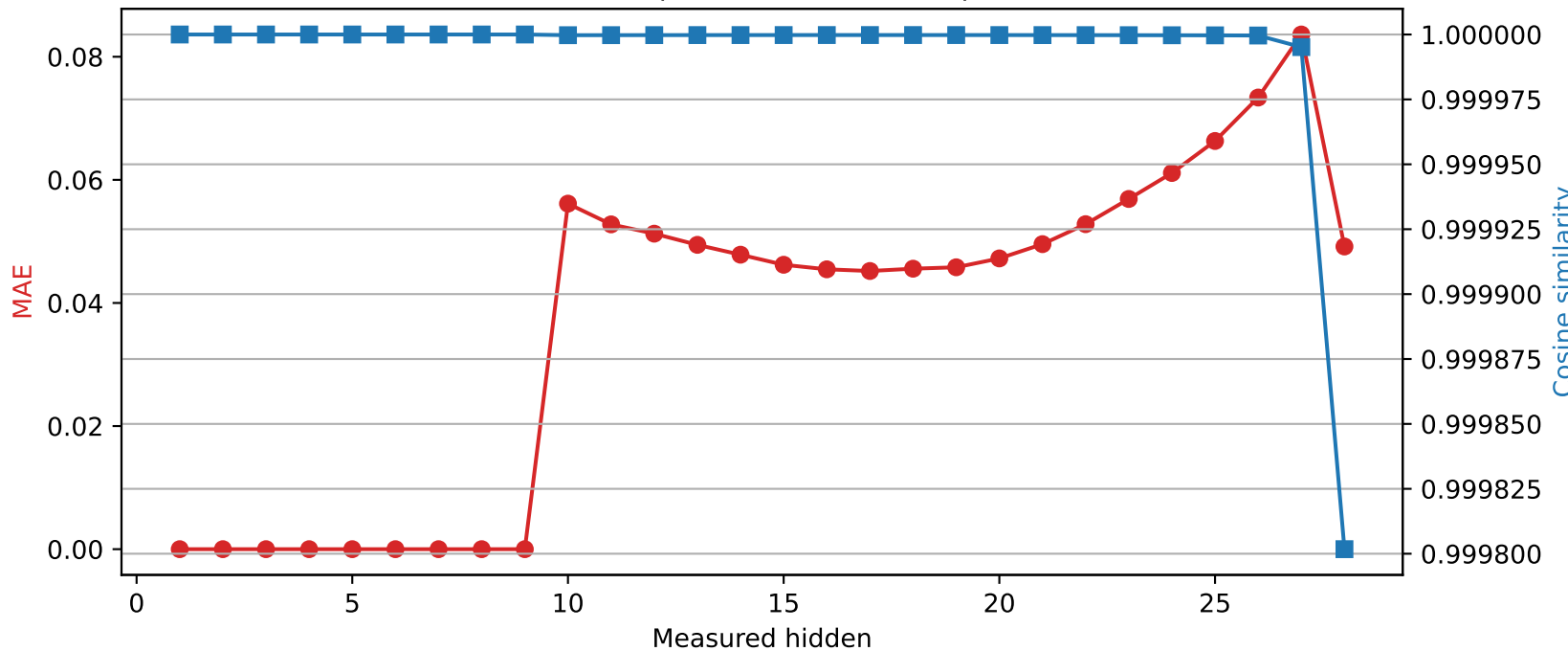
Qwen2.5-7B-Instruct | Quantized layer 9 | float16 \rightarrow int8
