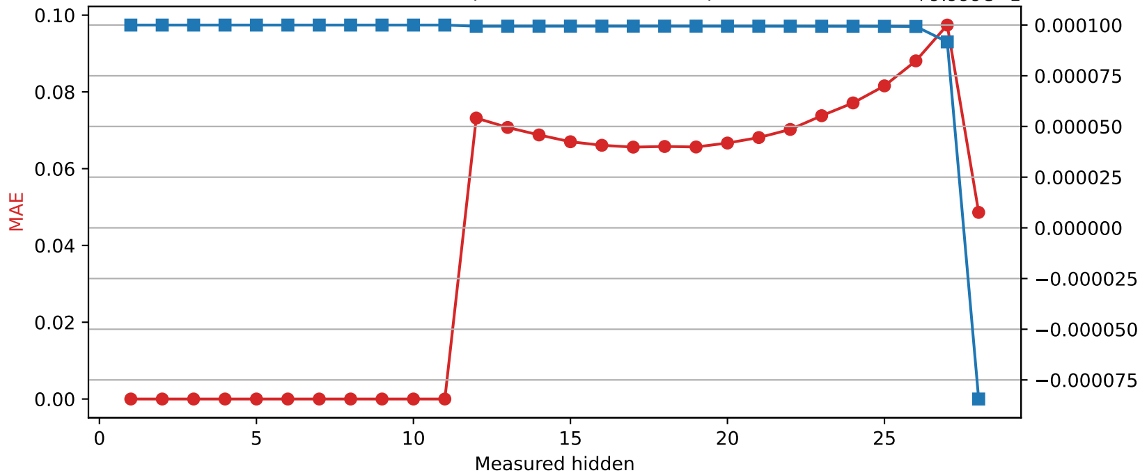
Qwen2.5-7B-Instruct | Quantized layer 11 | float16 → int8
