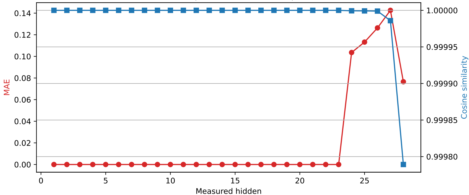
Qwen2.5-7B-Instruct | Quantized layer 23 | float16 → int8
