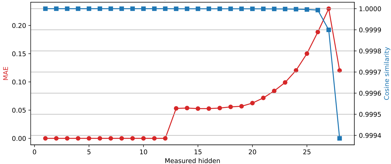
Qwen2.5-7B-Instruct | Quantized layer 12 | float16 → int8
