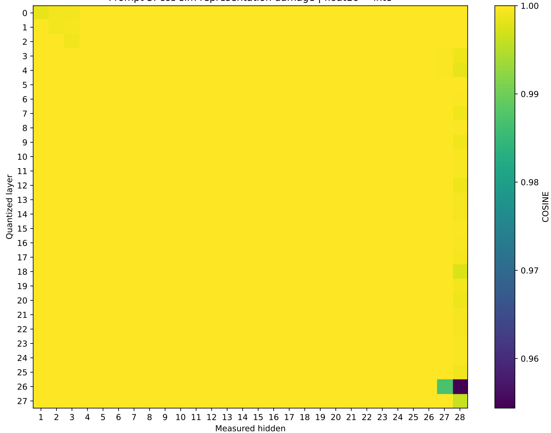
Qwen2.5-7B-Instruct Prompt 3: cos sim representation damage | float16 → int8
