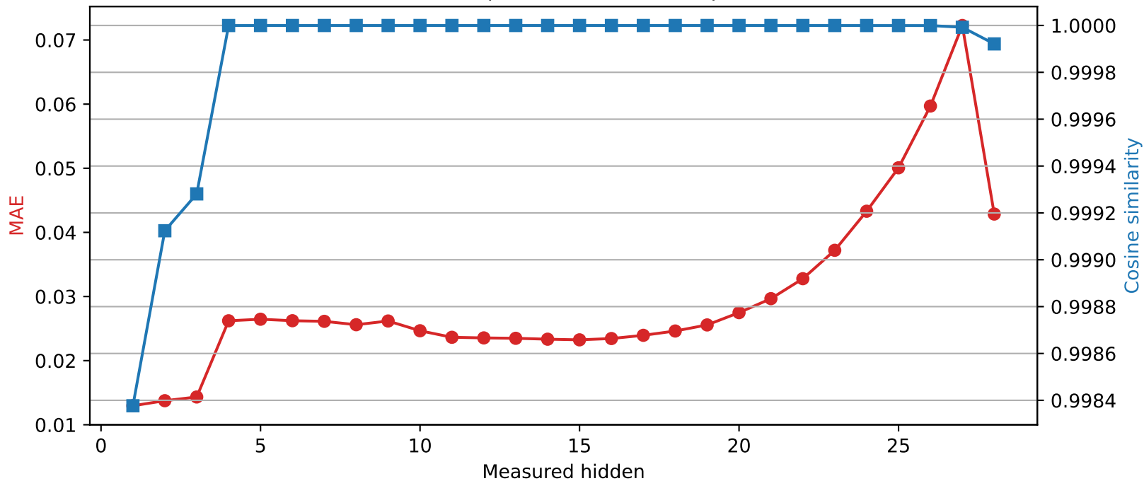
Qwen2.5-7B-Instruct | Quantized layer 0 | float16 → int8
