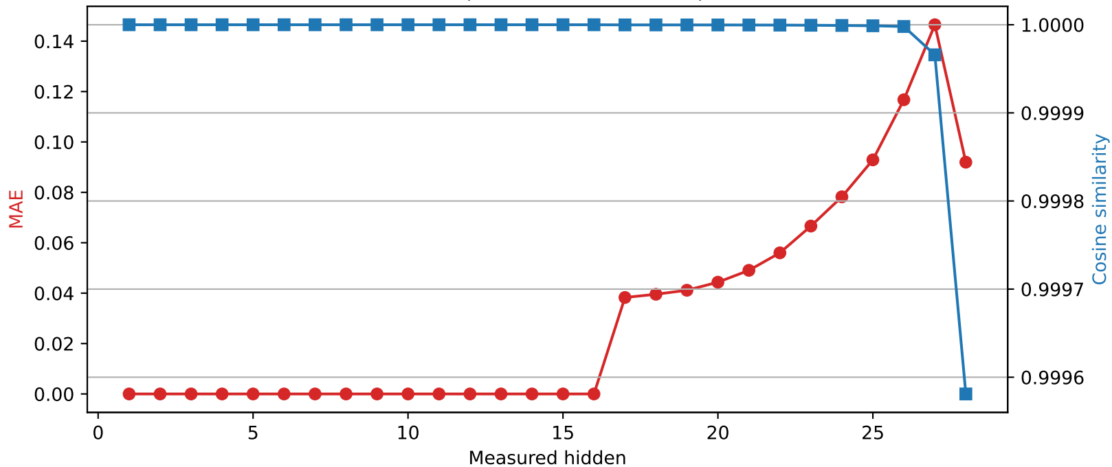
Qwen2.5-7B-Instruct | Quantized layer 16 | float16 → int8
