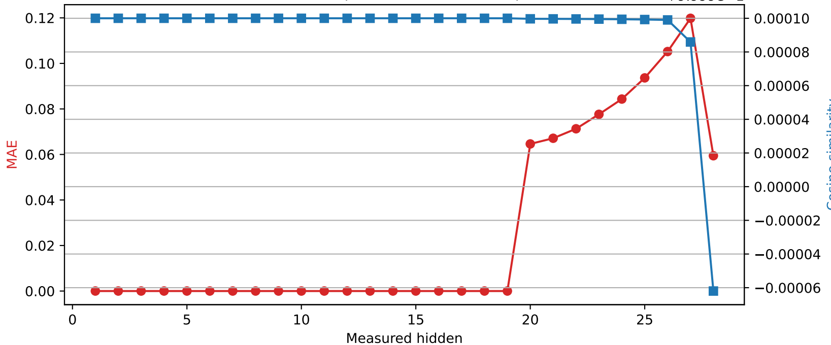
Qwen2.5-7B-Instruct | Quantized layer 19 | float16 \rightarrow int8
