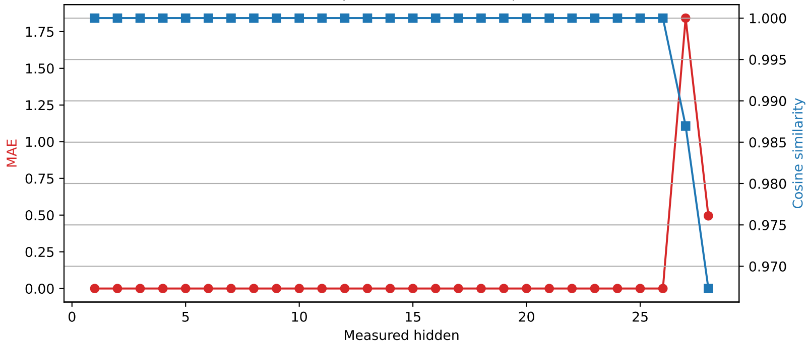
Qwen2.5-7B-Instruct | Quantized layer 26 | float16 → int8
