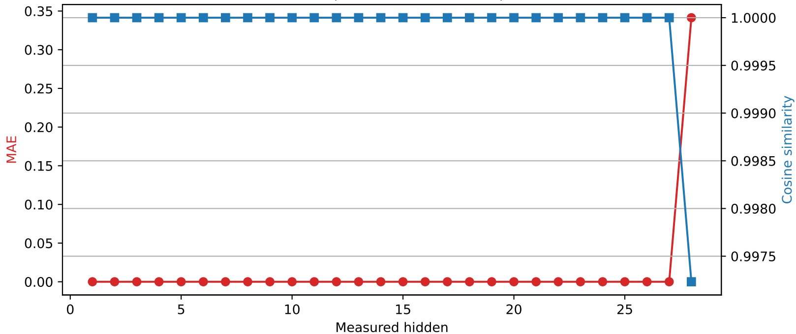
Qwen2.5-7B-Instruct | Quantized layer 27 | float16 \rightarrow int8
