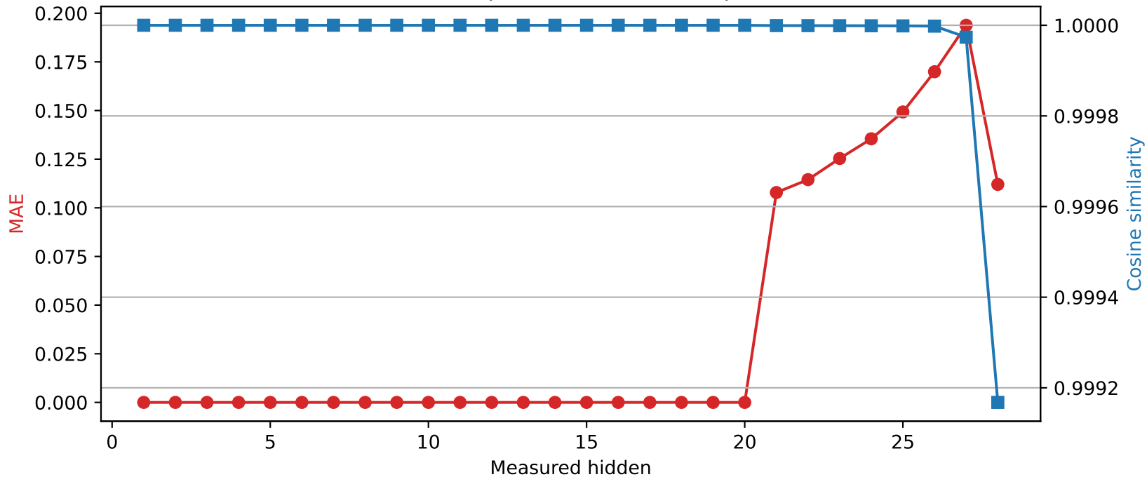
Qwen2.5-7B-Instruct | Quantized layer 20 | float32 \rightarrow int8
