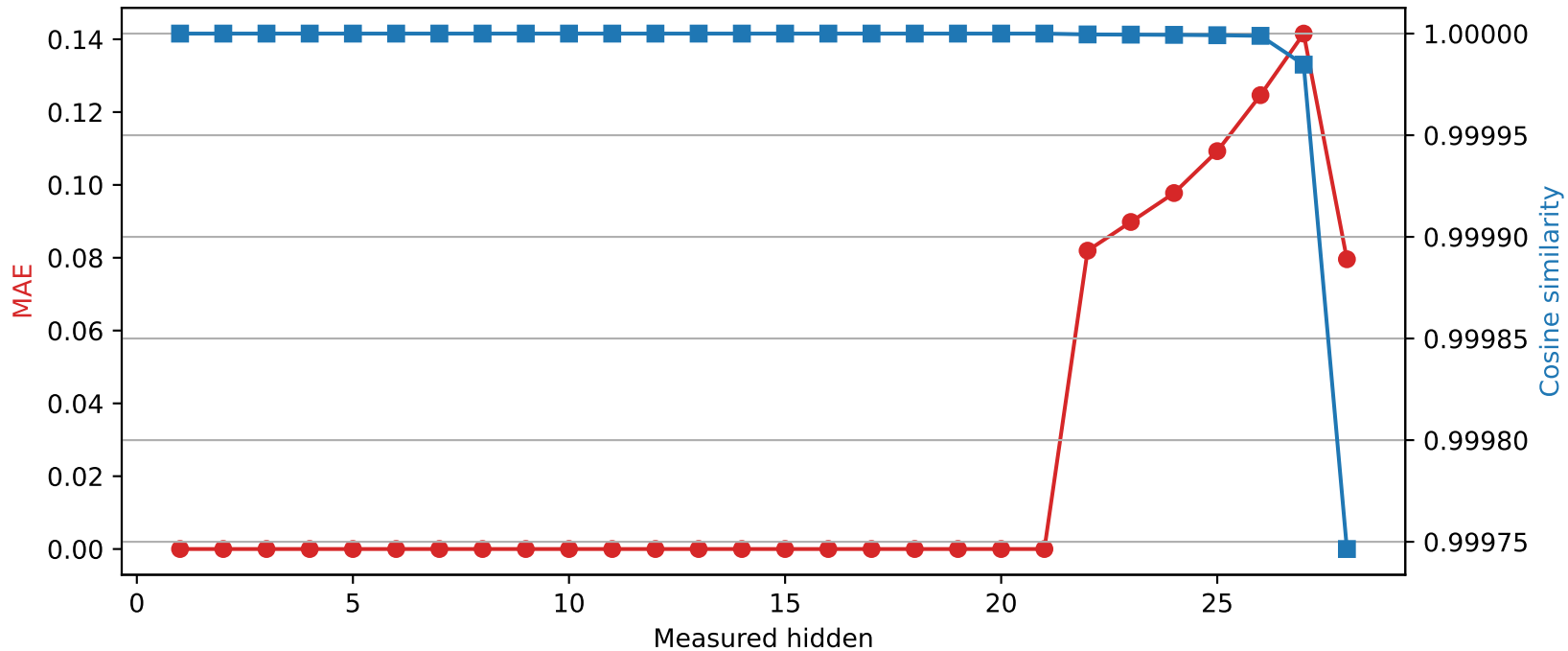
Qwen2.5-7B-Instruct | Quantized layer 21 | float32 → int8
