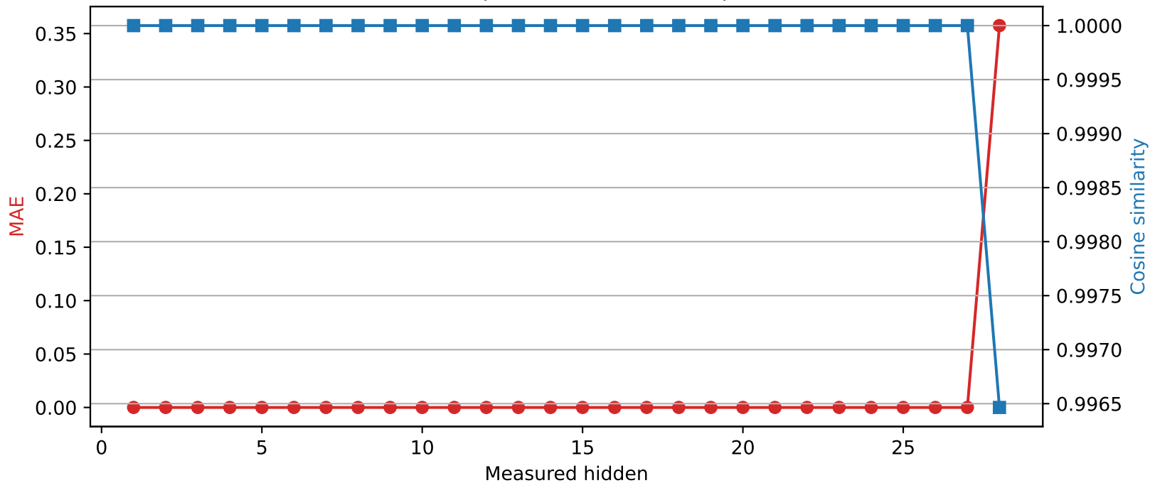
Qwen2.5-7B-Instruct | Quantized layer 27 | float32 → int8
