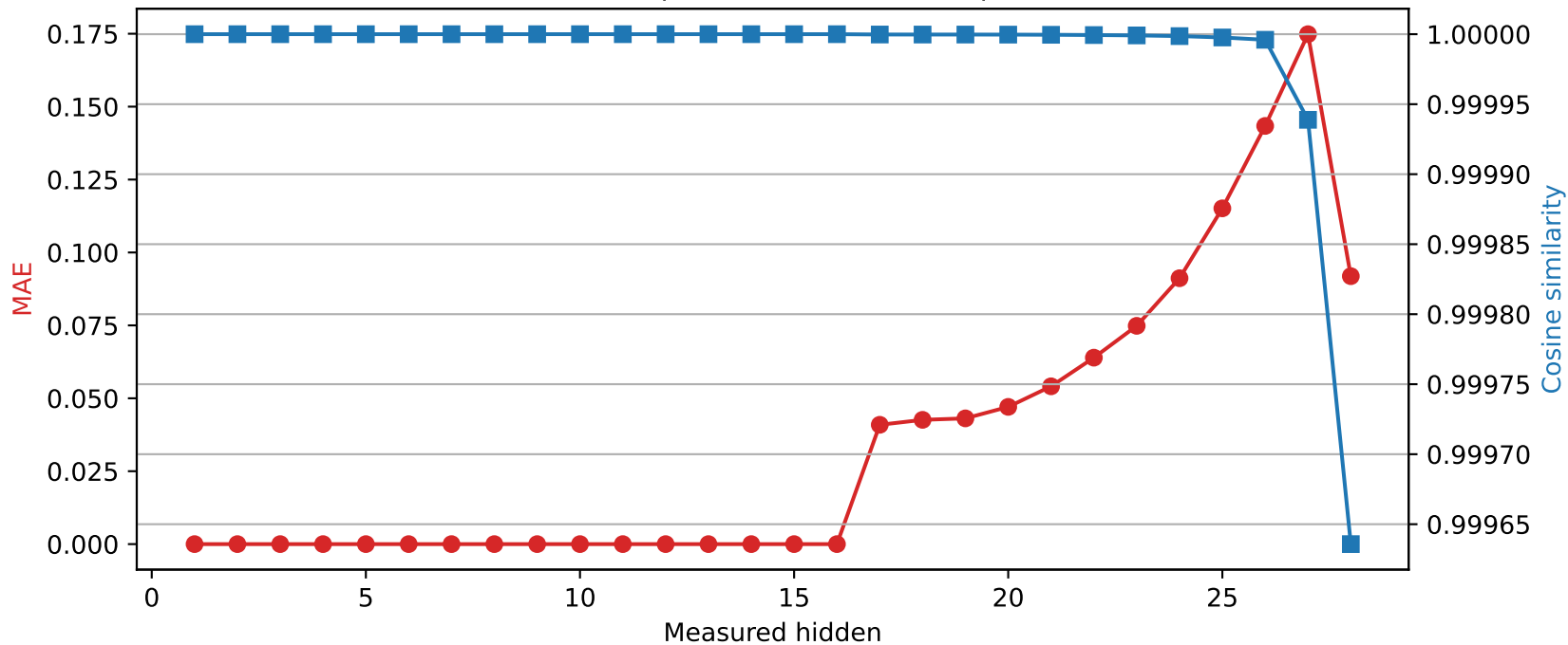
Qwen2.5-7B-Instruct | Quantized layer 16 | float32 → int8
