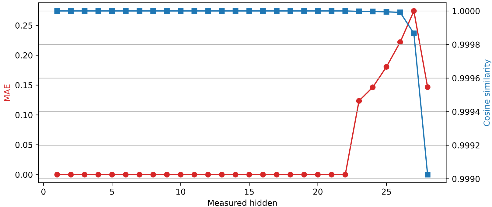
Qwen2.5-7B-Instruct | Quantized layer 22 | float32 \rightarrow int8
