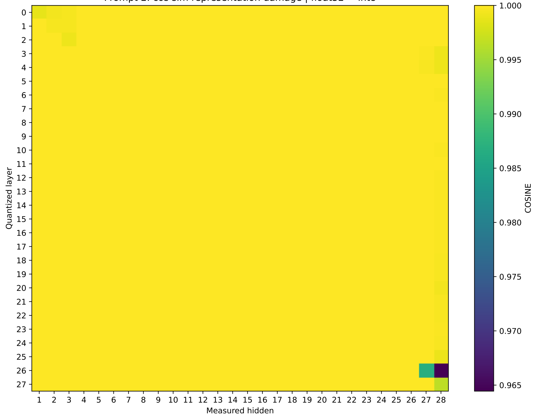
Qwen2.5-7B-Instruct Prompt 2: cos sim representation damage | float32 → int8
