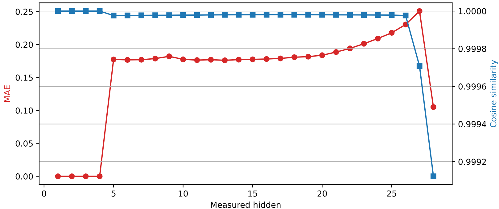
Qwen2.5-7B-Instruct | Quantized layer 4 | float32 → int8
