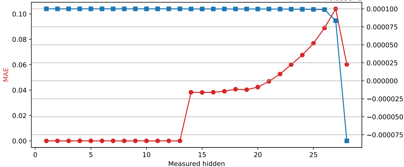
Qwen2.5-7B-Instruct | Quantized layer 13 | float32 \rightarrow int8
