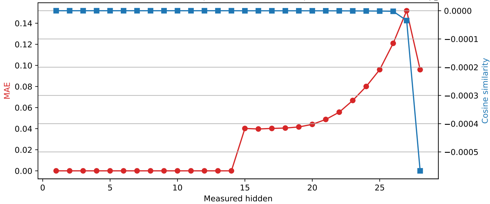
Qwen2.5-7B-Instruct | Quantized layer 14 | float32 \rightarrow int8
