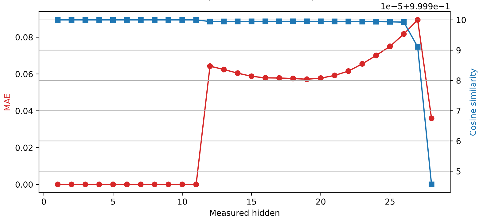
Qwen2.5-7B-Instruct | Quantized layer 11 | float32 → int8
