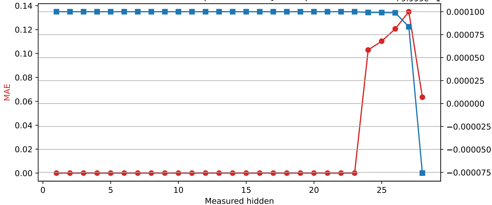
Qwen2.5-7B-Instruct | Quantized layer 23 | float32 → int8
