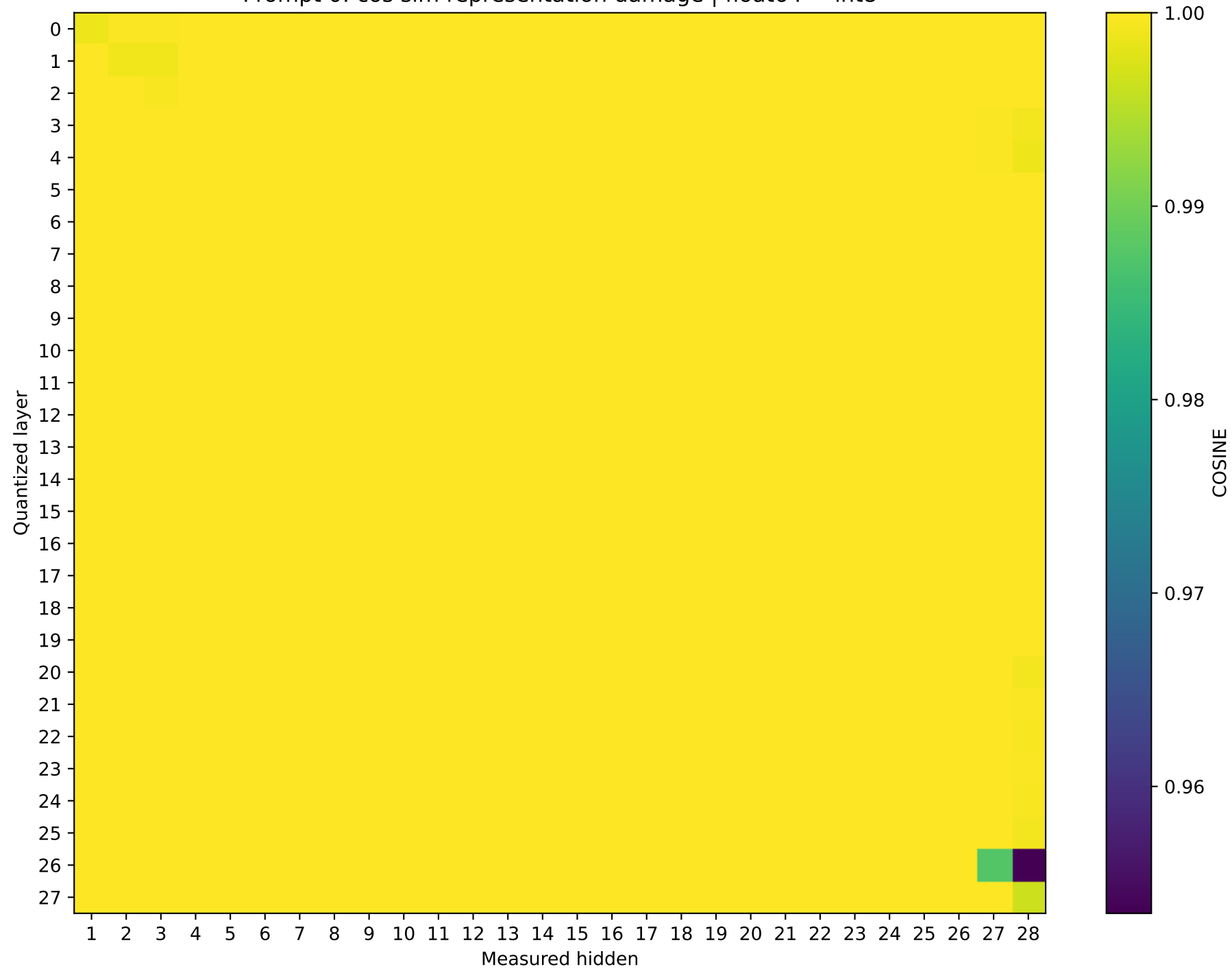
Qwen2.5-7B-Instruct Prompt 0: cos sim representation damage | float64 → int8
