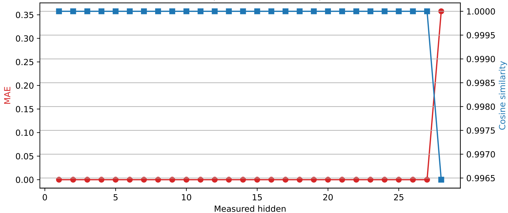
Qwen2.5-7B-Instruct | Quantized layer 27 | float64 → int8
