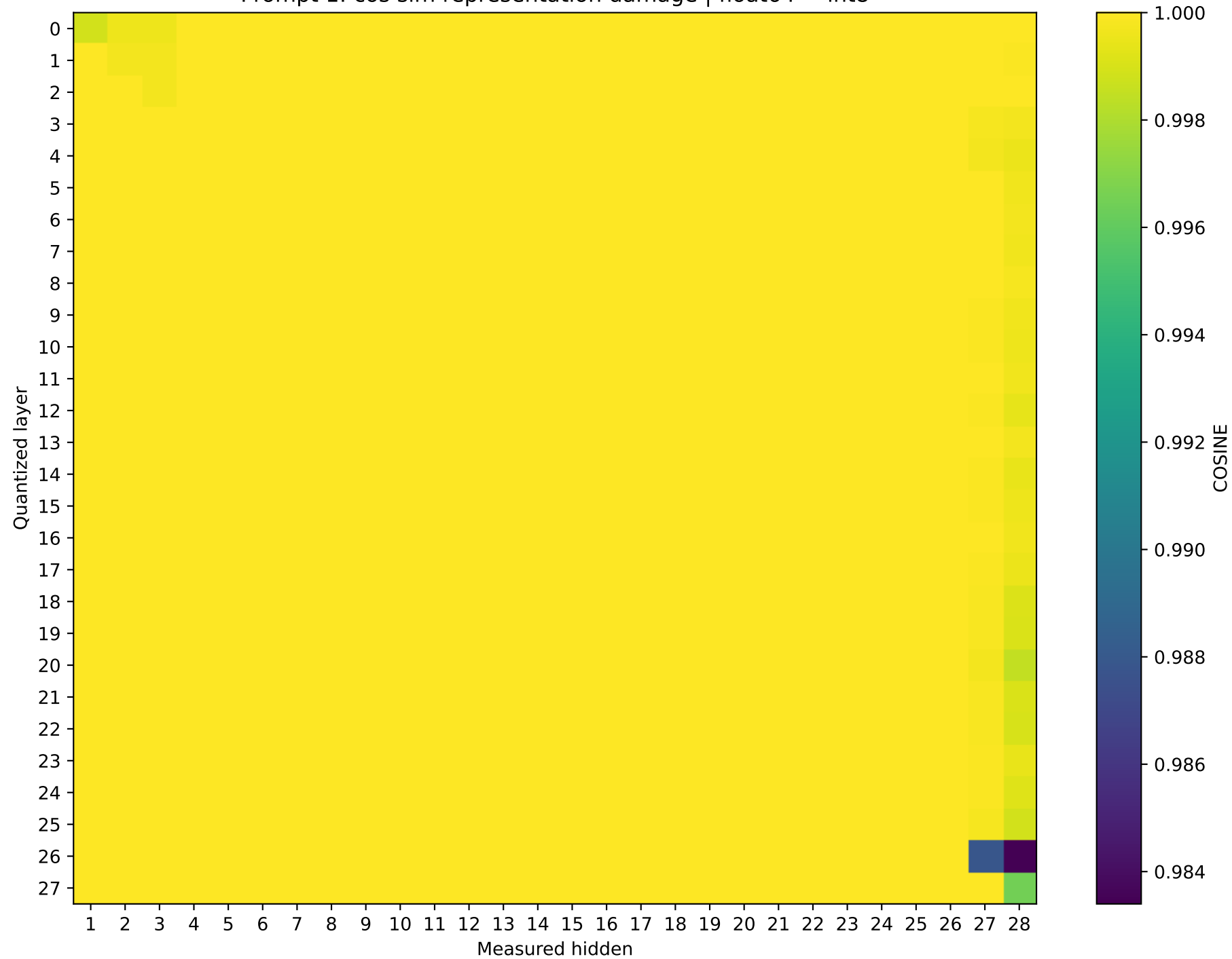
Qwen2.5-7B-Instruct Prompt 1: cos sim representation damage | float64 → int8
