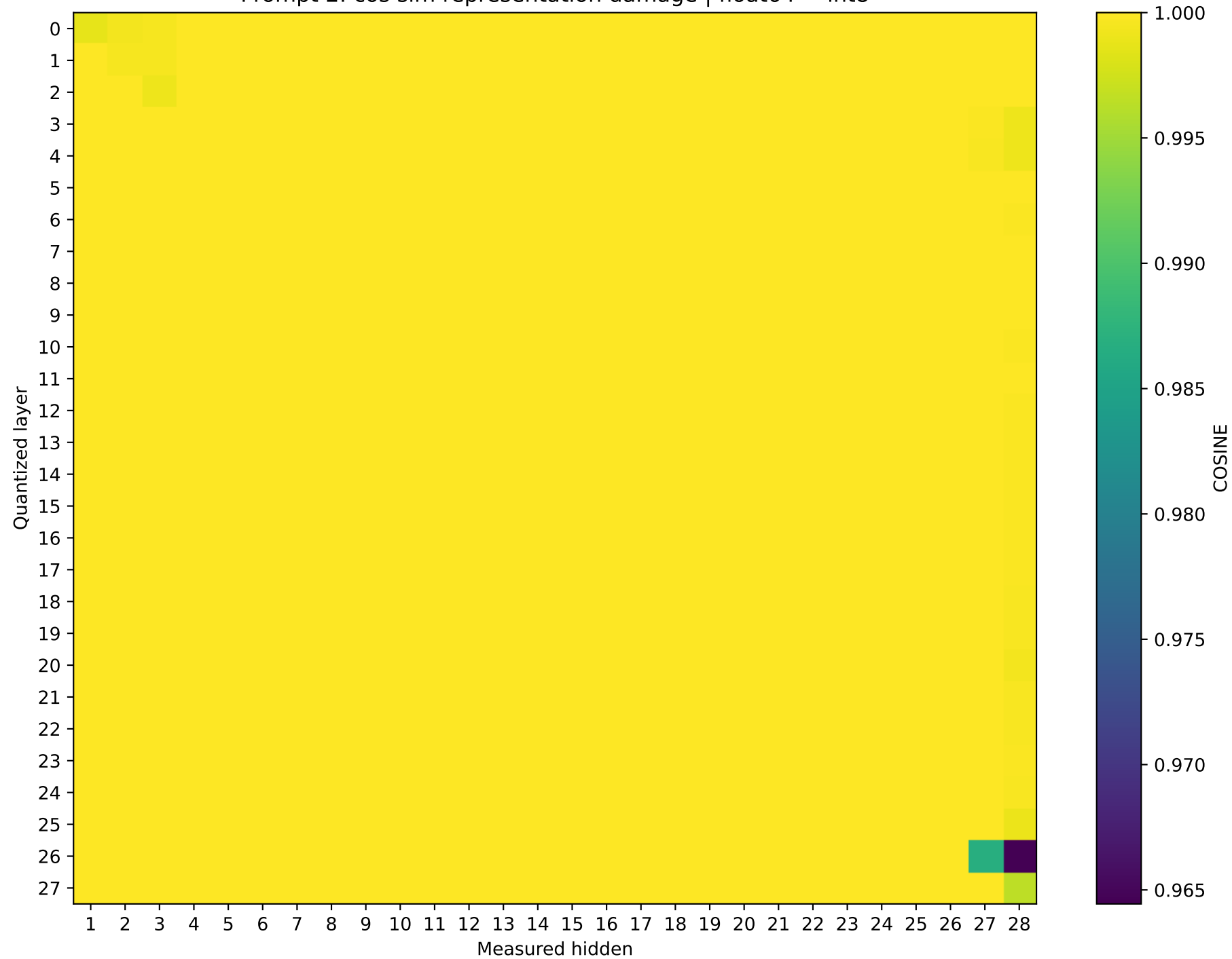
Qwen2.5-7B-Instruct Prompt 2: cos sim representation damage | float64 → int8
