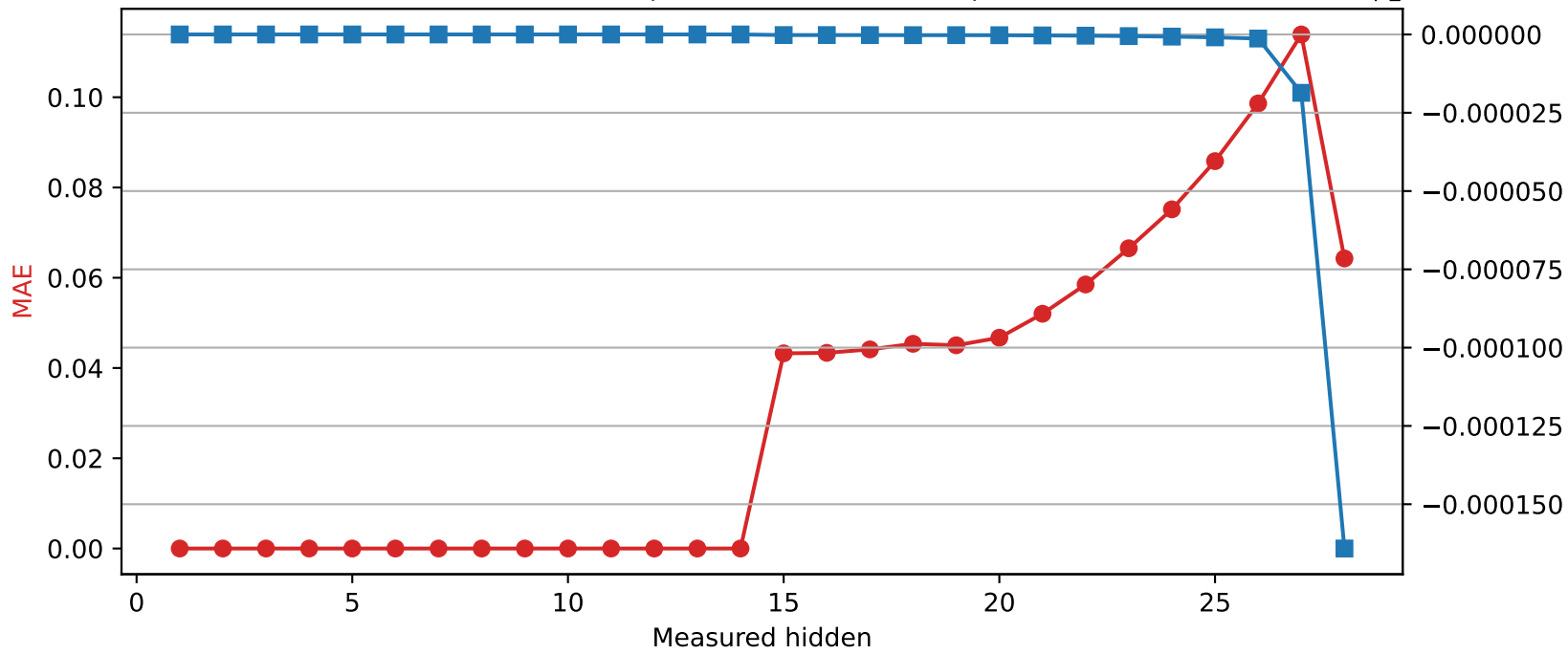
Qwen2.5-7B-Instruct | Quantized layer 14 | float64 → int8
