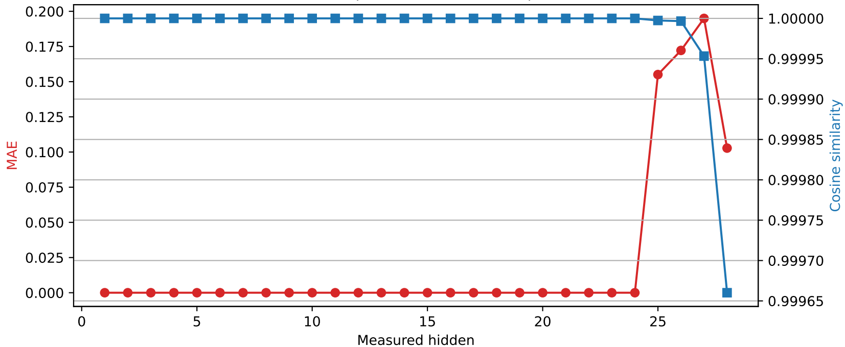
Qwen2.5-7B-Instruct | Quantized layer 24 | float64 → int8
