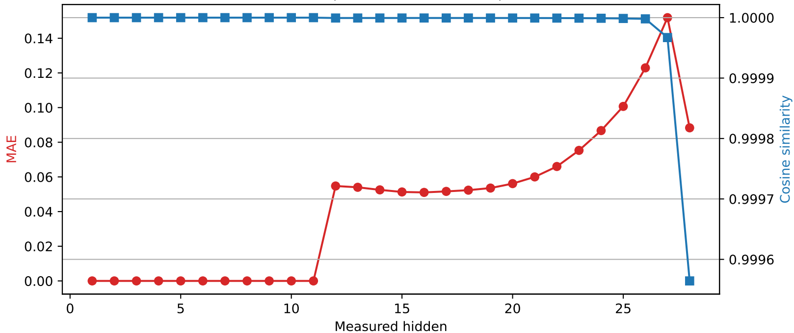
Qwen2.5-7B-Instruct | Quantized layer 11 | float64 → int8
