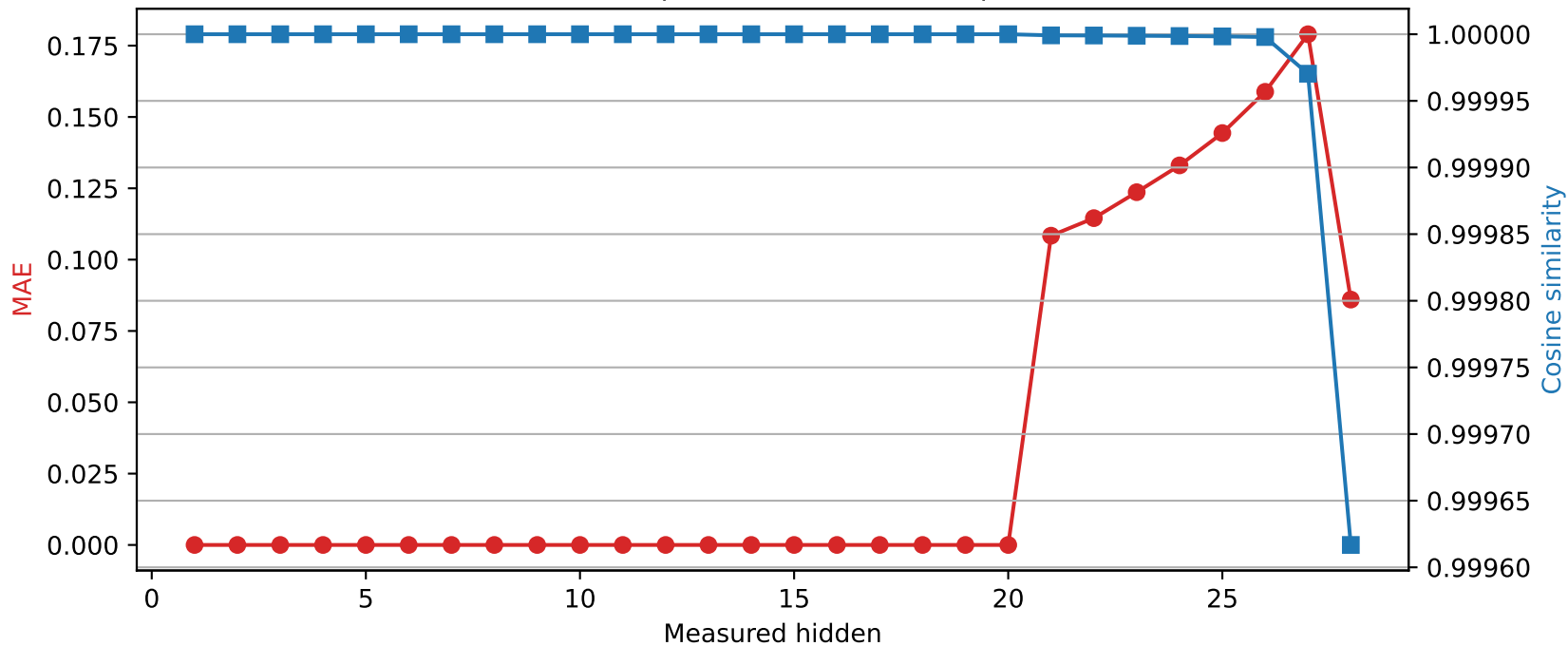
Qwen2.5-7B-Instruct | Quantized layer 20 | float64 → int8
