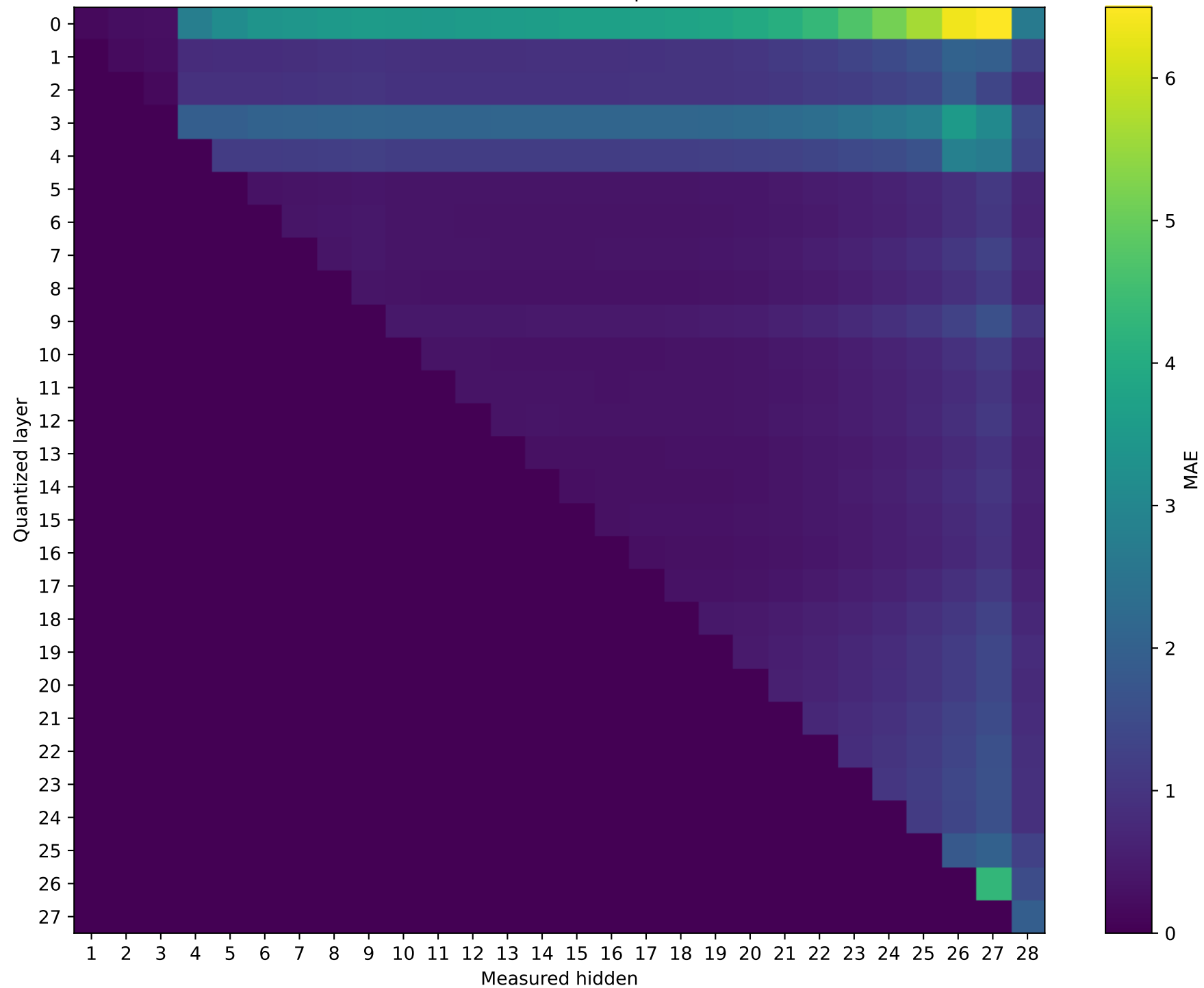
Model: Qwen2.5-7B-Instruct | float16 → int4
