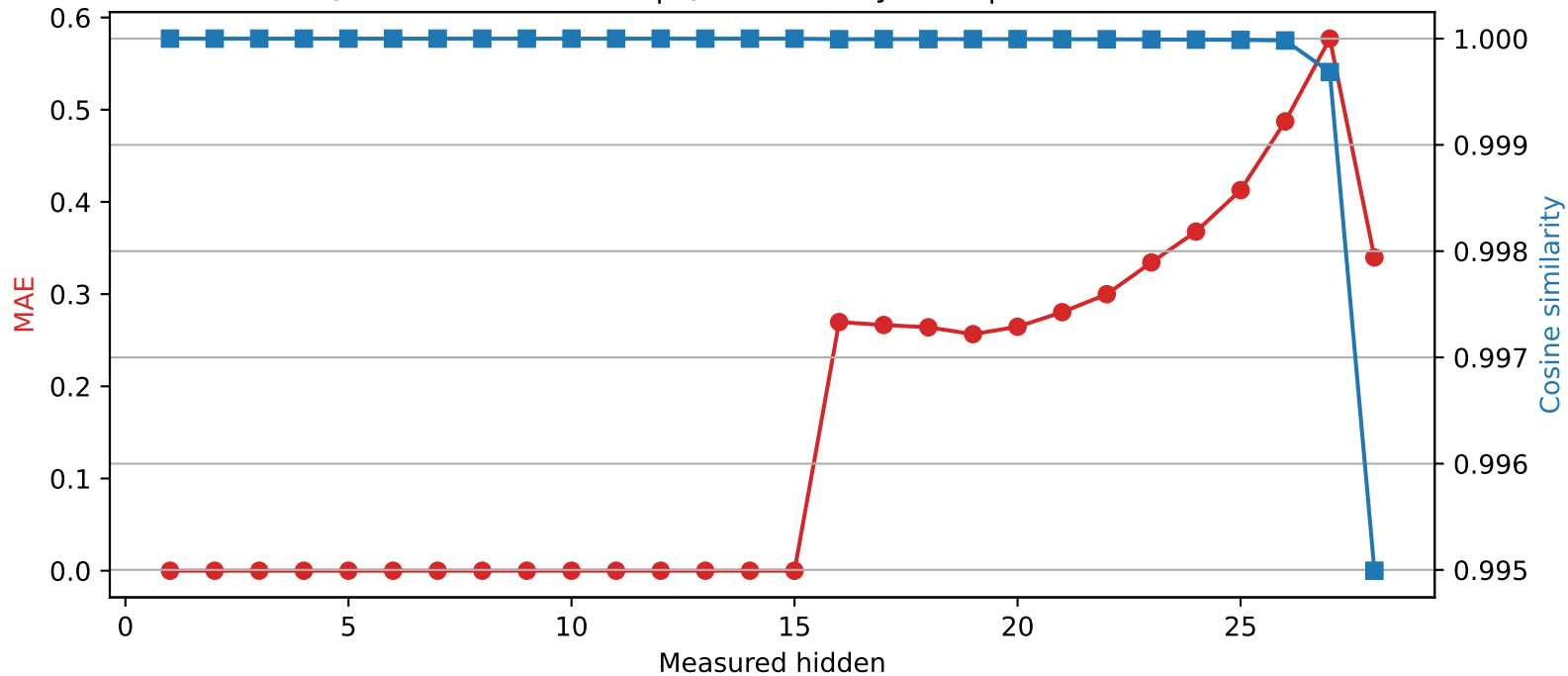
Qwen2.5-7B-Instruct | Quantized layer 15 | float16 → int4
