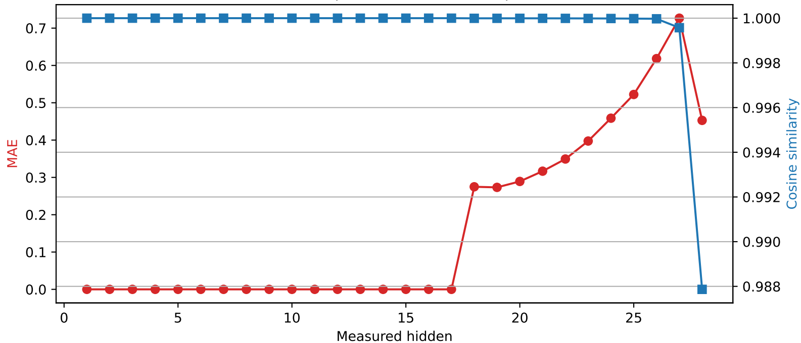
Qwen2.5-7B-Instruct | Quantized layer 17 | float16 \rightarrow int4
