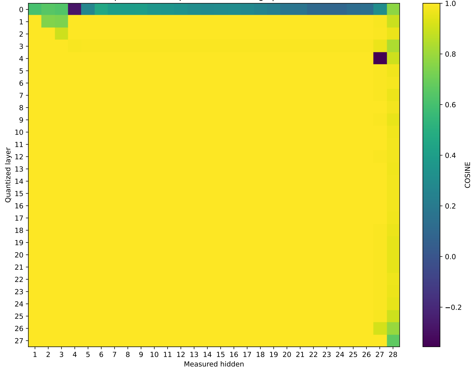
Qwen2.5-7B-Instruct Prompt 1: cos sim representation damage | float16 → int4
