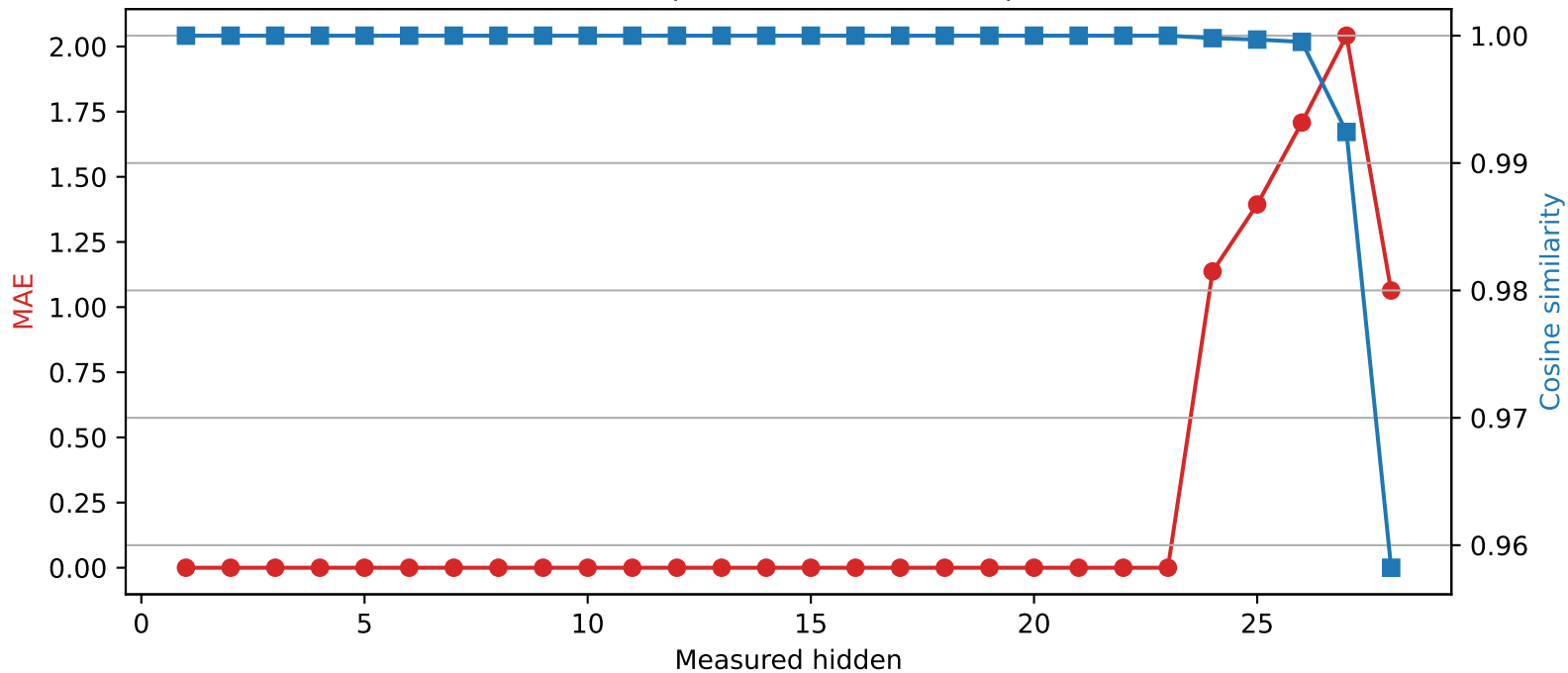
Qwen2.5-7B-Instruct | Quantized layer 23 | float16 \rightarrow int4
