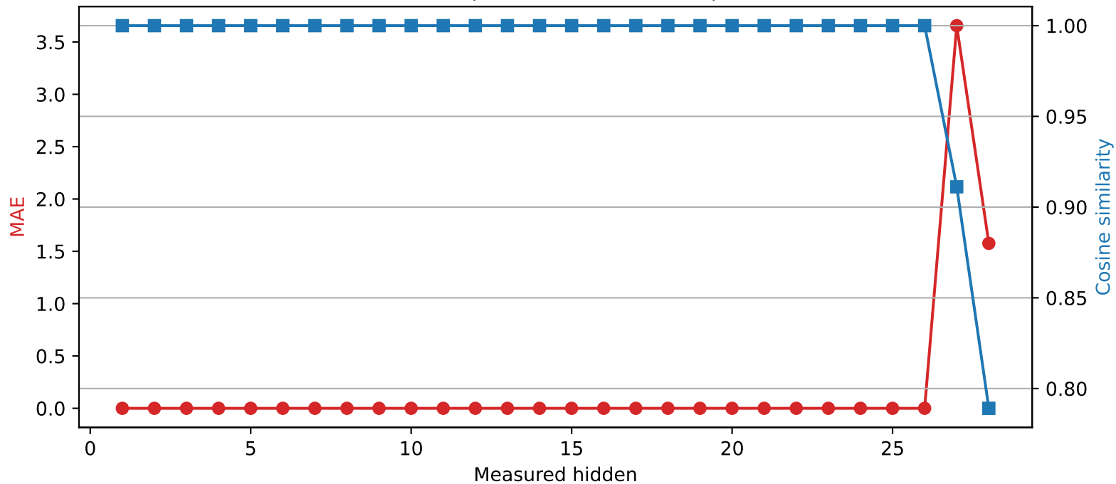
Qwen2.5-7B-Instruct | Quantized layer 26 | float16 \rightarrow int4
