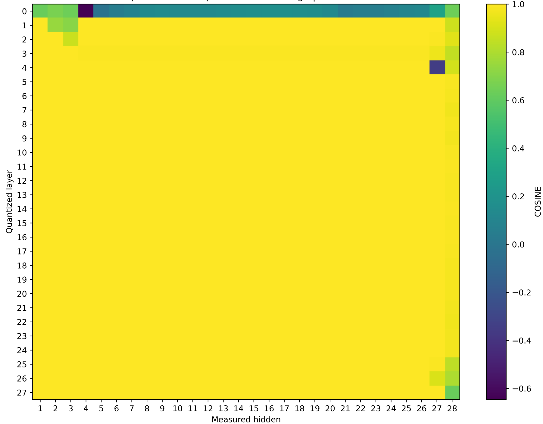
Qwen2.5-7B-Instruct Prompt 2: cos sim representation damage | float16 → int4
