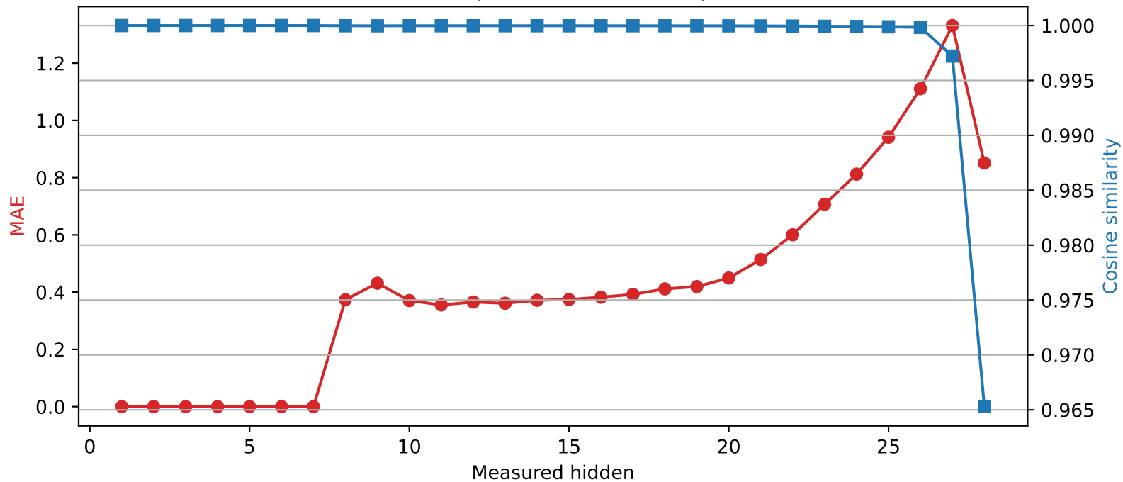
Qwen2.5-7B-Instruct | Quantized layer 7 | float16 → int4
