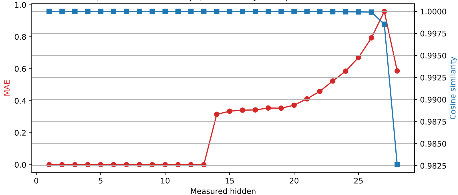
Qwen2.5-7B-Instruct | Quantized layer 13 | float16 → int4
