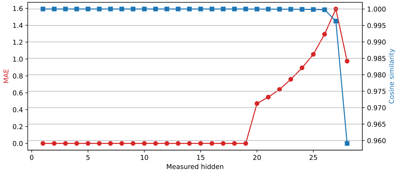
Qwen2.5-7B-Instruct | Quantized layer 19 | float16 → int4
