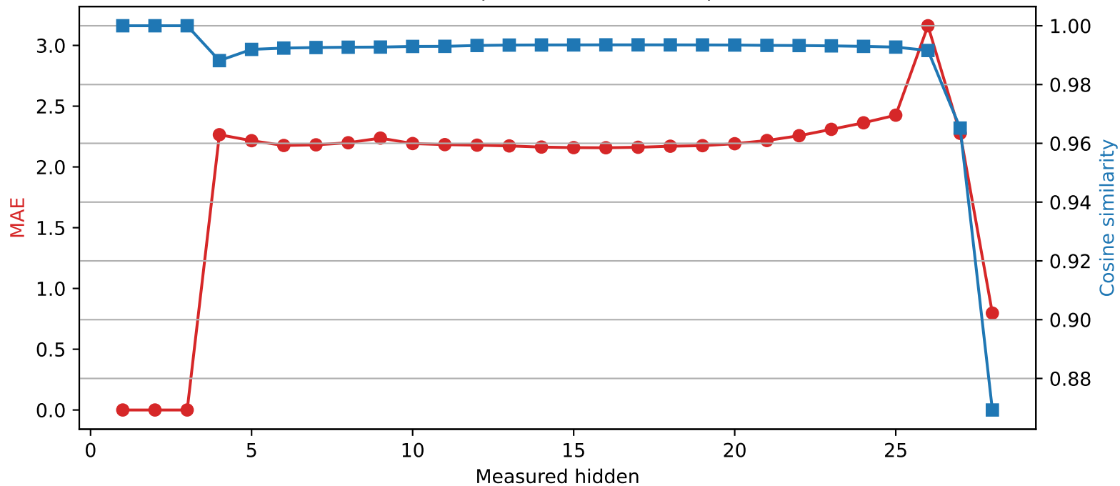
Qwen2.5-7B-Instruct | Quantized layer 3 | float16 → int4
